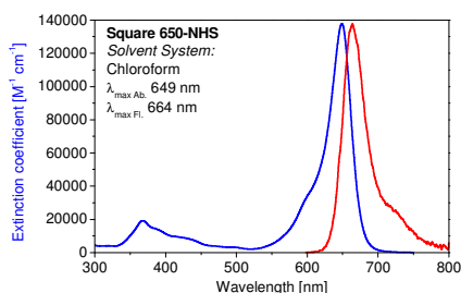
Absorption and fluorescence spectra of Square 650-NHS in chloroform
